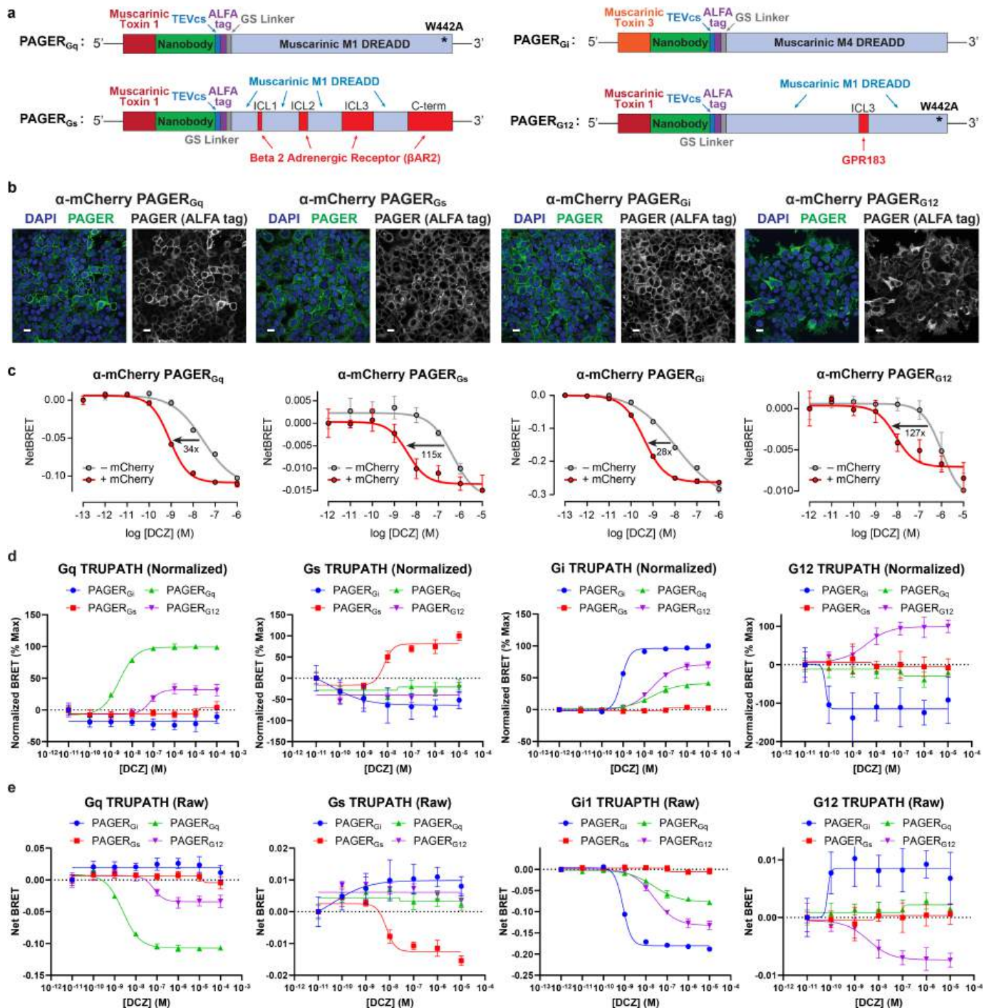
Extended Data Fig. 8 | Domain structures and characterization of PAGER c . a , Domain structures of optimized PAGER Gq , PAGER Gs , PAGER Gi , and PAGER G12 . The W442A mutation was found to improve membrane localization of M1 DREADD by reducing constitutive receptor internalization (Uwada et al., J Cell Sci , 2014) and thus introduced to both PAGER Gq and PAGER G12 . b , Immunofluorescence staining of HEK 293 T cells stably expressing PAGER c 's, using \alpha -ALFA-Alexa Fluor 647 (PAGER; green) and DAPI (nuclear stain; blue). Images are representative
