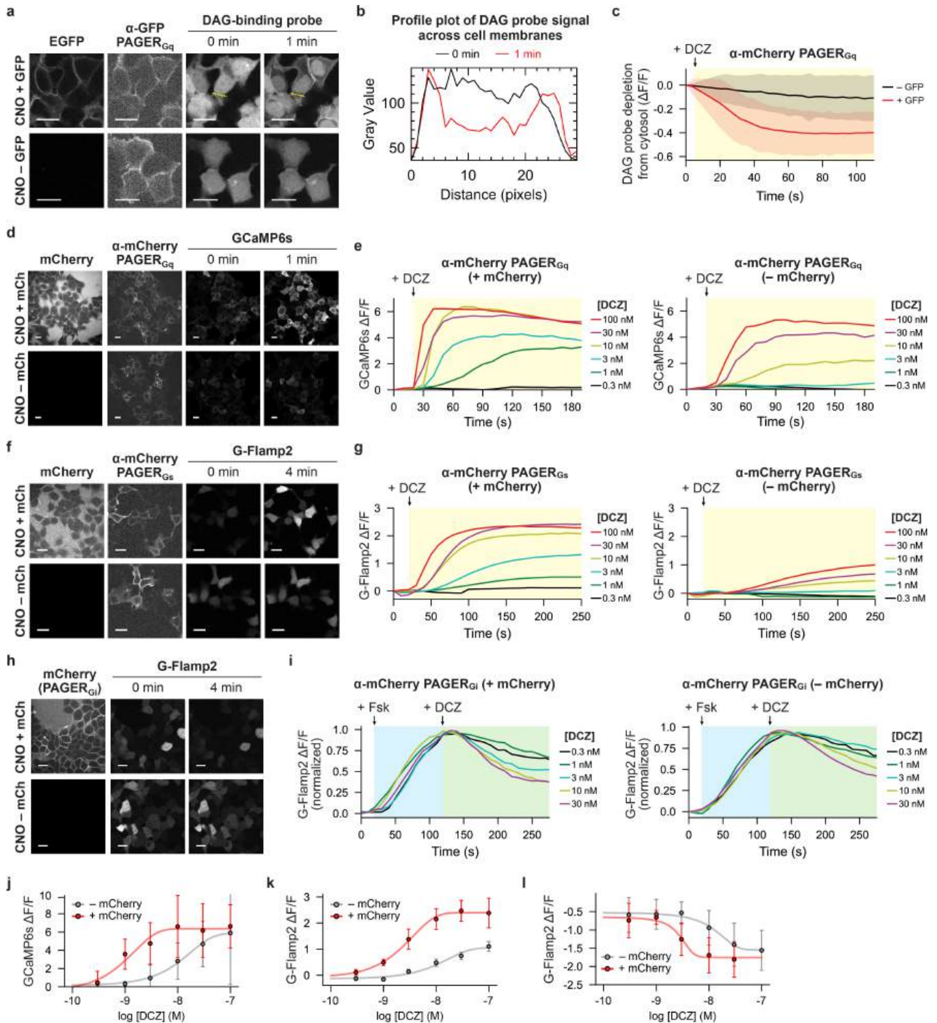
Extended Data Fig. 9 | Antigen-gated control of second messengers by PAGER c . a , Representative images showing antigen-dependent control of endogenous DAG lipid production with PAGER Gq . HEK cells expressing \alpha -GFP PAGER Gq and DAG probe were treated with 1 \mu M GFP and 100 nM CNO and imaged over time. b , Representative profile plot of DAG probe signal across cell membranes (marked by yellow dashed line in (a)), at t = 0 min (black) and t = 1 min (red). c , Time-course plot of experiment in (a). Plots show mean \pm s.d. for 28 and 27 individual cells, respectively, examined over n = 3 independent samples. d , Representative images showing antigen-dependent control of cytosolic Ca 2+ with PAGER Gq . HEK cells expressing \alpha -mCherry PAGER Gq and GCaMP6s 32 were preincubated with 2 \mu M mCherry for 3 min, stimulated with 100 nM CNO and imaged over time. e , Time-course plots of experiment in (d) at several different DCZ concentrations. f , Representative images showing
