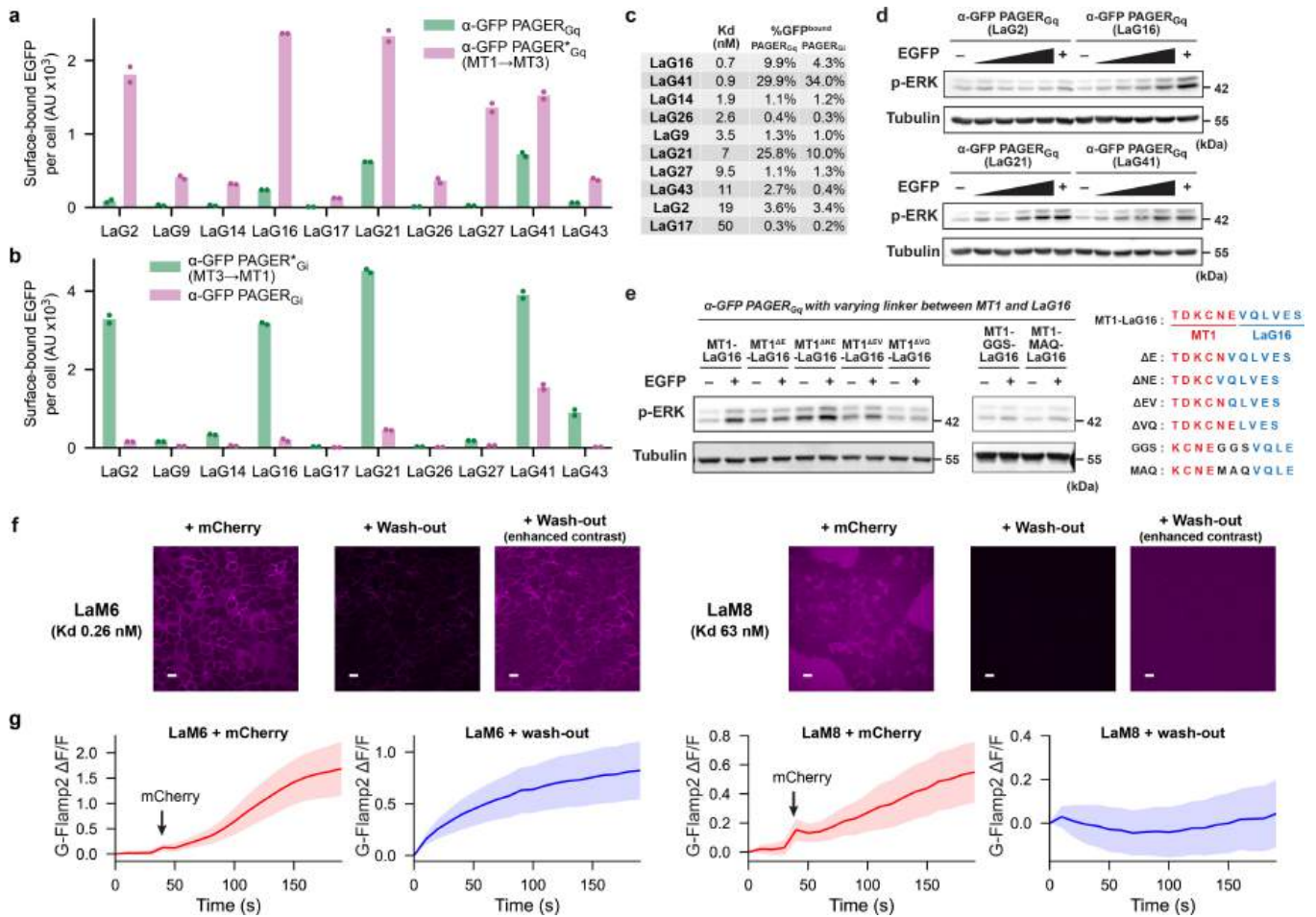
Extended Data Fig. 10 | Evaluation of different nanobodies and toxin truncations in PAGER Gq . a , Varying GFP nanobodies in original \alpha -GFP PAGER Gq (MT1-LaGx-hM1Dq; green) or in \alpha -GFP PAGER Gq * (MT3-LaGx-hM1Dq; magenta) where MT1 autoinhibitory domain was swapped with MT3 toxin. MT1 has higher reported affinity to M1 receptor than MT3. HEK cells expressing PAGER Gq with the indicated nanobody were treated with 10 \mu M GFP for 15 min, washed, and then analyzed by FACS. Quantitation was based on the average GFP signal per cell. Data representative of n = 2 biologically independent samples. b , Same assay as (a) but with \alpha -GFP PAGER Gq * (MT1-LaGx-hM4Di; green) and \alpha -GFP PAGER Gq (MT3-LaGx-hM4Di; magenta). MT3 has higher reported affinity to M4 receptor than MT1. Data representative of n = 2 biologically independent samples. c , Table summarizing reported affinities ( K_d ) of \alpha -GFP nanobodies along with the amount of GFP bound onto PAGER Gq (divided by the maximum amount of GFP bound in the lack of any antagonism). d , Western blots showing phosphorylation of endogenous ERK in response to GFP and CNO activation of PAGER Gq with four different GFP nanobodies. HEK cells expressing the indicated
