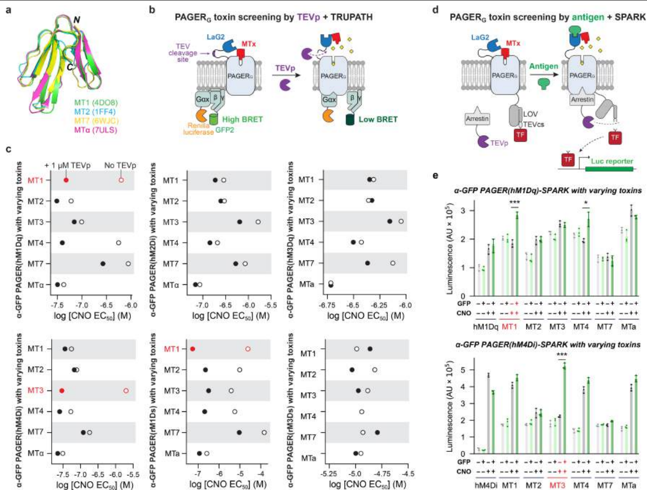
Extended Data Fig. 7 | Screening muscarinic toxins in PAGER G for conditional auto-inhibition. a , Overlay of muscarinic toxins that have experimentally-solved structures (PDB accession code: MT1, 4DO8; MT2, 1FF4; MT7, 6WJC; MT \alpha , 7ULS). b , Schematic of TRUPATH BRET assay used to screen PAGER G constructs containing various muscarinic toxins (MTs). 1 \mu M recombinant TEV protease (TEVp) was added for 90 min prior to CNO addition to relieve auto-inhibition. c , Results of TRUPATH screen, showing EC 50 values for CNO, with and without TEVp pre-treatment. The rMID-based PAGER G have ICL2-3 from rM3D grafted into hM1Dq. The constructs colored red showed the best dynamic range and were selected as the final PAGER G 's. Full CNO dose-response curves
