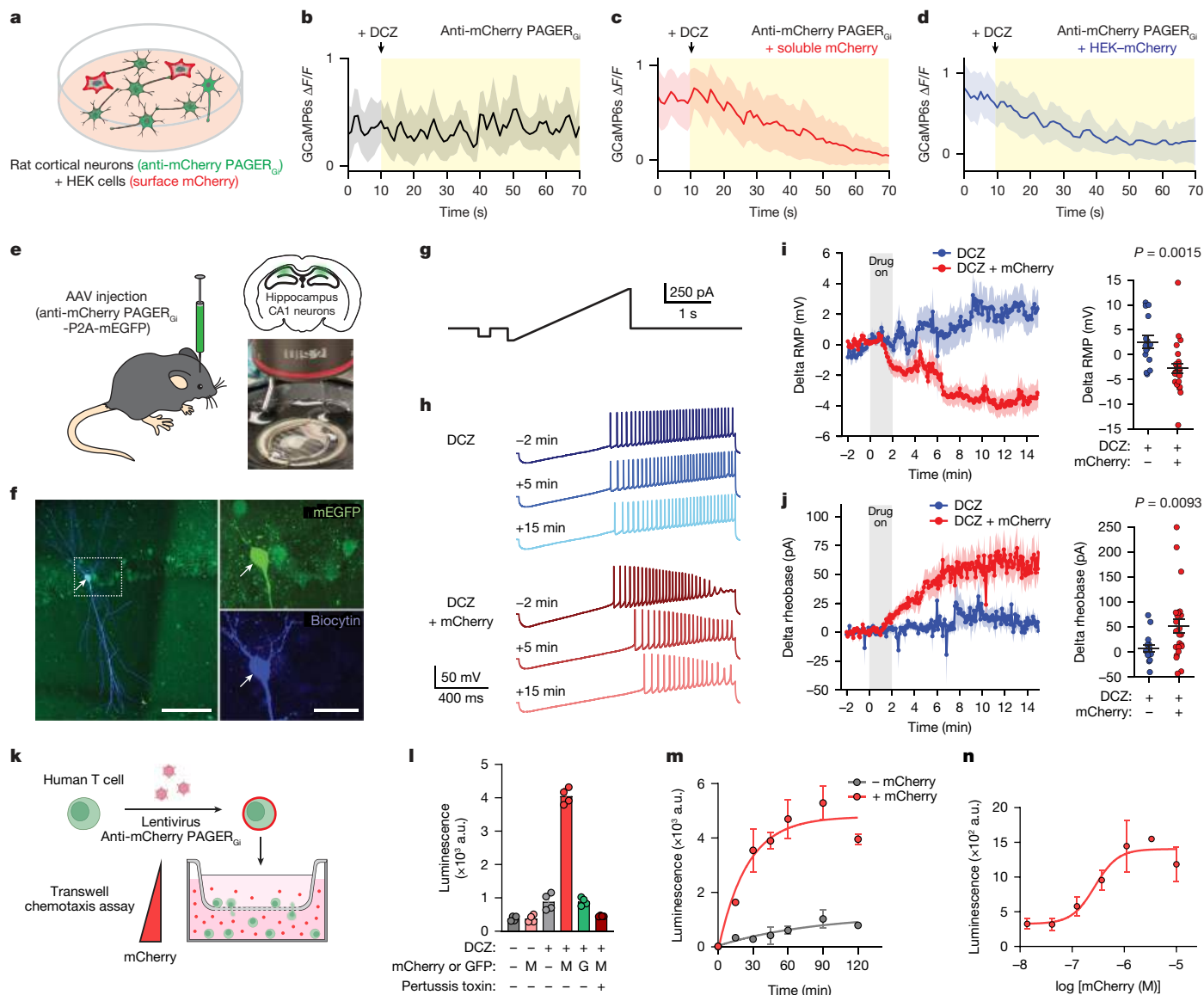
Fig. 4 | PAGER Gi controls diverse cell behaviours in acute brain slices and primary T cells. a , Schematic of co-culture experiment for PAGER Gi control of neuronal activity. b–d , Calcium traces in rat cortical neurons co-expressing anti-mCherry PAGER Gi and GCaMP6s with or without soluble (1 μM) or surface mCherry. DCZ was added at t = 10 s to a final concentration of 2 nM. Data are mean ± s.d. for n = 50 cells from 3 independent experiments. e , Schematic for PAGER Gi -mediated neuronal inhibition in acute brain slices. f , Maximum intensity projection showing mEGFP labelling in PAGER Gi -expressing neurons in CA1 (representative of n = 14 assessed cells). Biotin labelling shows a recorded neuron (arrow). Scale bar: left, 100 μm; right, 30 μm. g , Current clamp protocol for monitoring intrinsic electrical property dynamics of PAGER Gi -expressing neurons. h , Representative traces of evoked action potential alterations following DCZ (100 nM) with or without mCherry (1 μM) application. Neurons displayed greater intrinsic property shifts associated with reduced excitability when presented with DCZ plus mCherry rather than DCZ alone. i, j , Changes in
