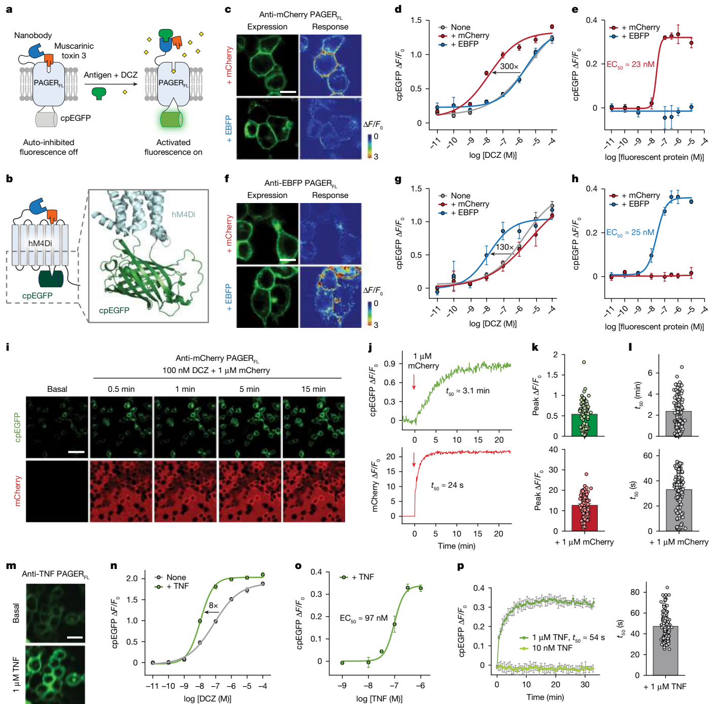
Fig. 5 | PAGER FL for real-time fluorescence detection of extracellular antigens. a , Schematic of PAGER FL , based on GRABs 1,2 . PAGER FL activation results in GPCR conformational changes, causing increased fluorescence of an inserted cpEGFP. b , Schematic and model structure of cpEGFP insertion between helices 5 and 6 in PAGER FL . c , Representative images of expression and response of anti-mCherry PAGER FL after 30 min treatment with 100 nM DCZ and 1 μM mCherry or EBFP (control). Scale bar, 10 μm. d , DCZ dose–response curves for anti-mCherry PAGER FL ± 1 μM mCherry or EBFP. n = 300 cells from 3 independent experiments. Data are mean ± s.e.m. e , Antigen dose–response of anti-mCherry PAGER FL with mCherry or EBFP and 100 nM DCZ. n = 300 cells from 3 independent experiments. Data are mean ± s.e.m. f–h , As c–e , but with anti-EBFP PAGER FL . Scale bar, 10 μm. Data are mean ± s.e.m. i , Representative images of anti-mCherry PAGER FL at various timepoints after 1 μM mCherry addition. n = 3 independent experiments. Scale bar, 50 μm. j , Time traces of
