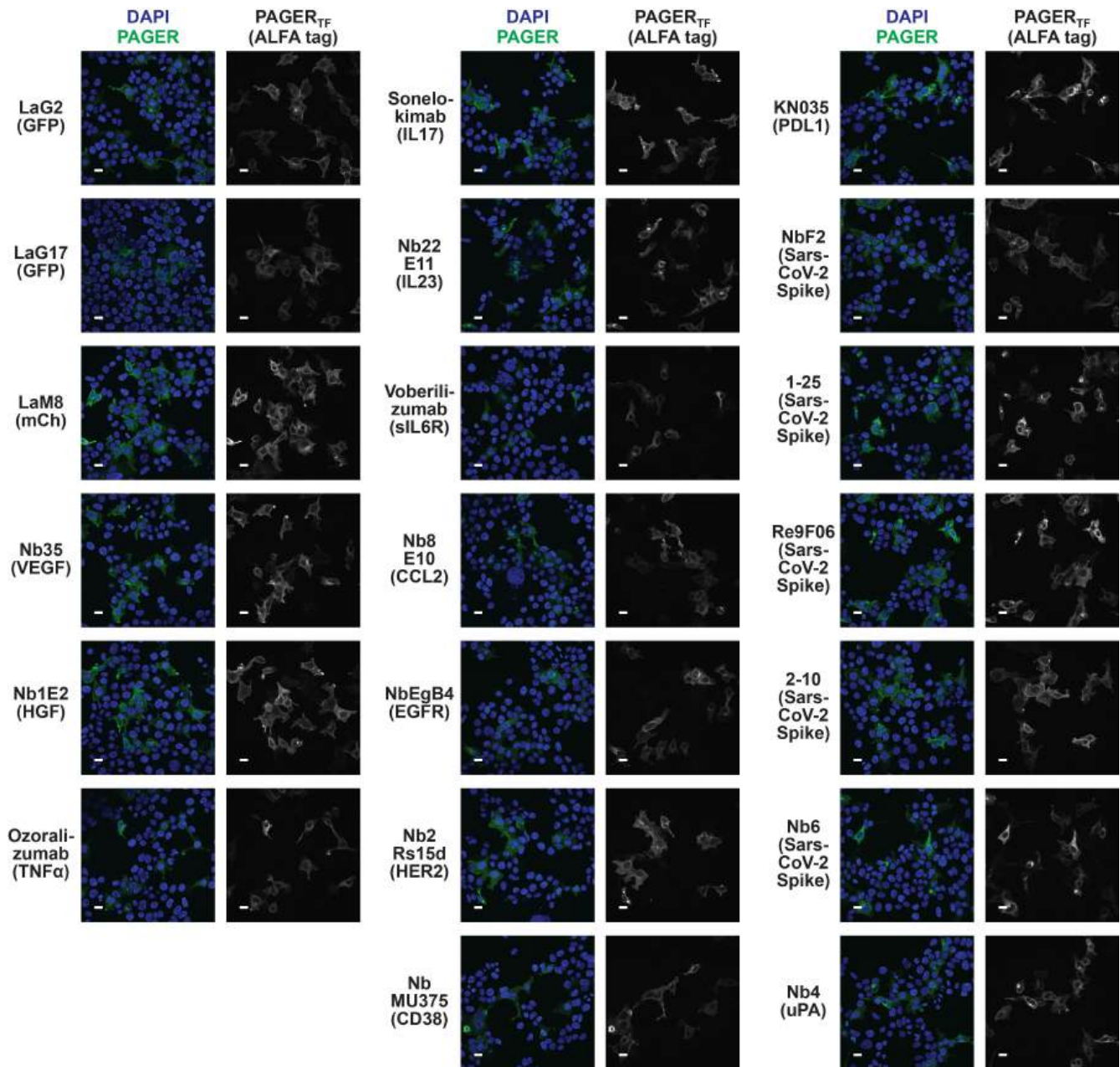
Extended Data Fig. 4 | Imaging PAGER TF expression and membrane localization. Immunofluorescence staining of fixed and permeabilized HEK 293 T cells transiently expressing PAGER TF with the indicated nanobody (target
