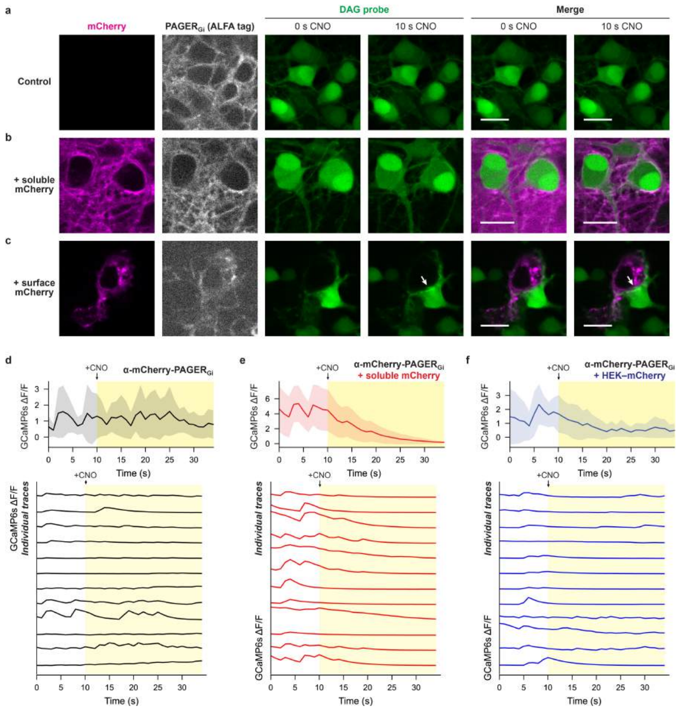
Extended Data Fig. 11 | PAGER Gi mediates antigen-dependent control of neuronal activity in culture. a–c , Representative images of antigen-gated DAG production in neurons. Rat cortical neurons expressing α-mCherry PAGER Gi and DAG probe (C 1 PKC Y -mCherry 31 ) were stimulated with 100 nM CNO and imaged over time. In (b), neurons were preincubated with 1 μM mCherry (no washout). In (c), HEK cells expressing surface mCherry (pink) were plated on top of neurons. Note the DAG probe accumulation at sites of HEK-neuron contact (arrowheads). Scale bars, 20 μm. Similar results were obtained in three
