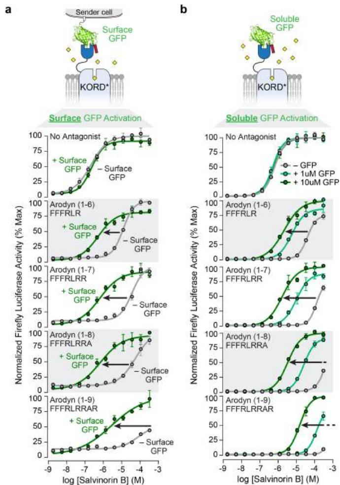
Extended Data Fig. 2 | Testing PAGER TF with different antagonist peptides for response to surface or soluble GFP antigen. a , SalB dose response curves for various PAGER TF constructs with or without co-culture with surface GFP-expressing sender cells. b , SalB dose response curves for various PAGER TF constructs with or without soluble GFP. Data presented here shows the same data (normalized) that is shown in Fig. 1k-l (update callouts) but with additional arodyn peptide antagonists included. Plots are mean \pm s.d. for 3 technical replicates per condition, n = 1 independent experiment.
