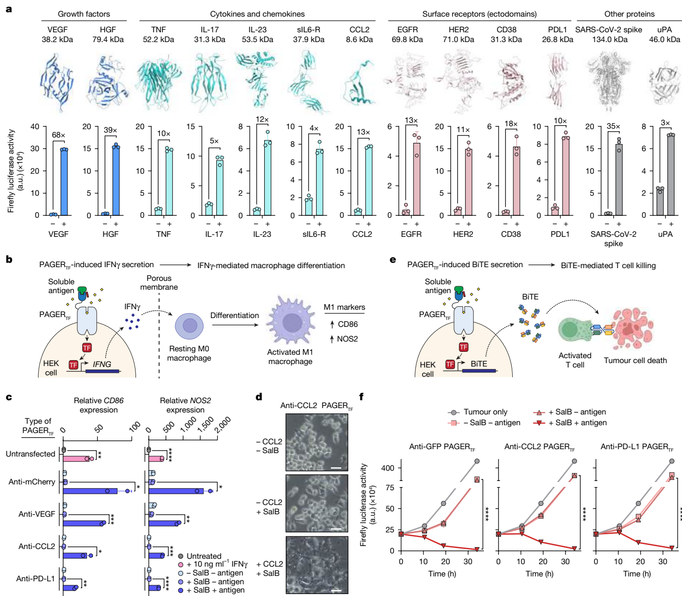
Fig. 2 | PAGER TF can detect a wide variety of antigens. a , Top, ribbon structures of proteins sensed by PAGER TF . Bottom, bar graphs of PAGER TF activity in response to cognate antigen. Antigen and SalB concentrations are reported in Methods. For anti-VEGF, anti-TNF, anti-IL-17 and anti-uPA PAGERS, n = 3 independent experiments, 3 replicates per condition. For all other PAGERS, n = 2 independent experiments, 3 replicates per condition. Data are mean \pm s.d. Two-tailed Student's t -test. b , Schematic of PAGER TF -driven macrophage differentiation in co-culture. PAGER TF activation in HEK293T cells induces the secretion of mouse IFN \gamma which passes through a porous membrane and stimulates M1 macrophage differentiation. c , Relative expression of M1 macrophage markers CD86 and NOS2 in co-cultured RAW 264.7 macrophages, determined by quantitative PCR (qPCR). n = 3 experiments, 2 replicates per condition. Data are mean \pm s.d.
