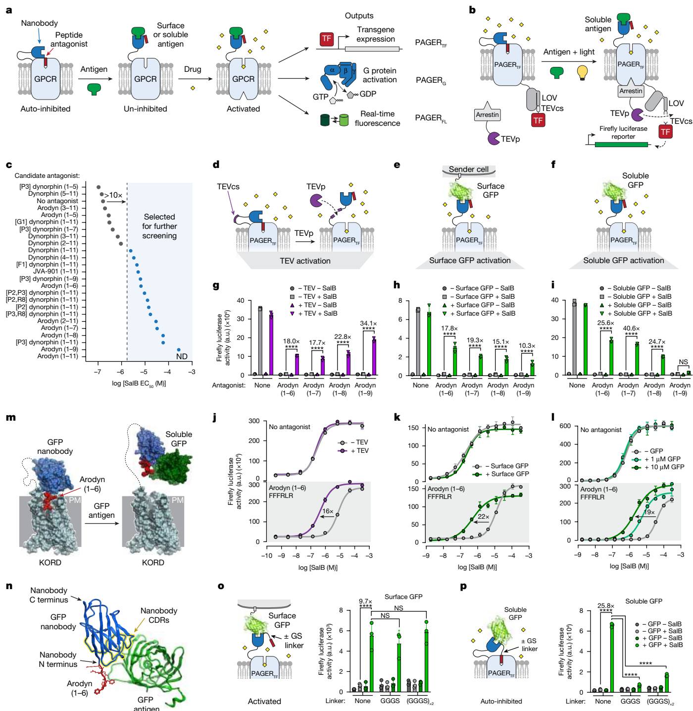
Fig. 1 | Design and optimization of PAGER. a , PAGER overview. Auto-inhibition by fused peptide antagonist is relieved by antigen binding and allows drug activation of the GPCR. PAGER activation can drive transgene expression (PAGER TF ), G-protein activation (PAGER G ) or real-time fluorescence (PAGER FL ). TF, transcription factor. b , Schematic of PAGER TF . PAGER-driven transgene expression based on SPARK 14,15 (specific protein association tool giving transcriptional readout with rapid kinetics). PAGER TF activation results in proteolytic release of a tethered transcription factor. LOV, light-, oxygen- and voltage-sensitive domain. c , Summary of SalB EC 50 values for candidate antagonist peptides screened in PAGER TF . n = 3 independent experiments, 3 replicates per condition. ND, not defined. d–f , Schematics for PAGER TF activation by extracellular TEVp ( d ), surface-expressed GFP ( e ) or soluble GFP ( f ). g–i , PAGER TF activity in response to SalB and TEV treatment ( g ), co-plating with HEK cells presenting surface GFP ( h ) or soluble GFP ( i ). n = 3, 5 or 4 independent experiments, respectively, 3 replicates per condition. Data are mean ± s.d. Two-way ANOVA with Tukey’s multiple comparisons test. j–l , SalB dose–response curves for PAGER TF activity with arodyn (1–6) antagonist and TEV pretreatment ( j ), co-plating with HEK cells presenting surface GFP ( k ) or soluble GFP ( l ). n = 5, 2 or 2 independent experiments, respectively, 3 replicates per condition. Data are mean ± s.d. m , AlphaFold2 model of antagonism and antigen-dependent relief of antagonism in PAGER. PM, plasma membrane. n , AlphaFold2 model highlighting proximity between the CDRs (yellow) and N terminus of the nanobody, where the antagonist peptide (red) is fused. o , PAGER TF variants with flexible Gly-Ser linkers can be activated by surface GFP expressed on co-plated HEK 293T cells. n = 3 independent experiments, 3 replicates per condition. Data are mean ± s.d. (two-way ANOVA with Tukey’s multiple comparisons test). p , PAGER TF variants with flexible Gly-Ser linkers cannot be activated by soluble GFP. n = 3 independent experiments, 3 replicates per condition. Data are mean ± s.d. Two-way ANOVA with Tukey’s multiple comparisons test. * P < 0.05, ** P < 0.01, *** P < 0.001, **** P < 0.0001; NS, not significant.
