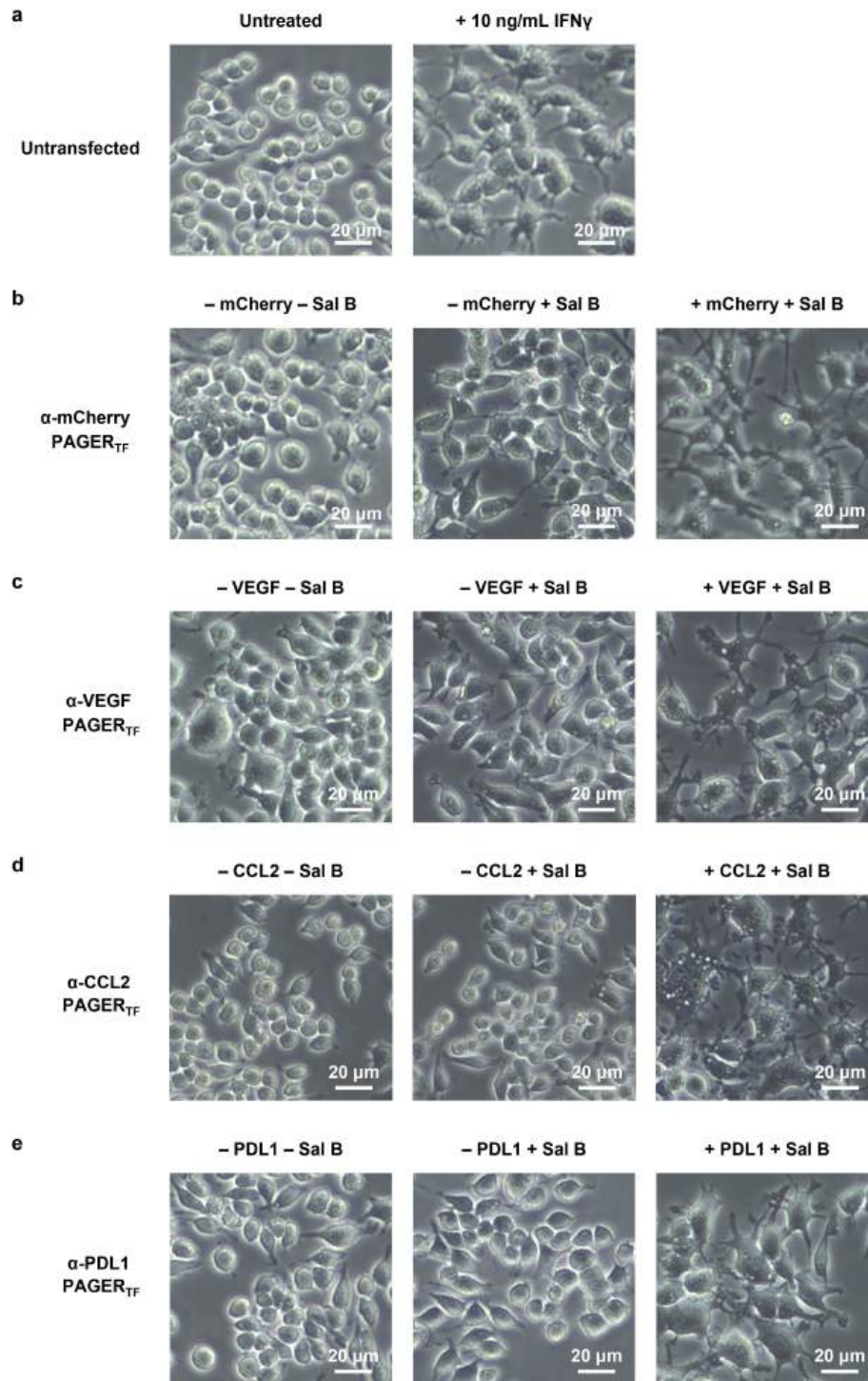
Extended Data Fig. 6 | PAGER TF -induced IFN \gamma drives macrophage differentiation (Related to Fig. 2b-d). Representative images of Raw 264.7 macrophages after 48 h of co-culture with the indicated PAGER TF -expressing
