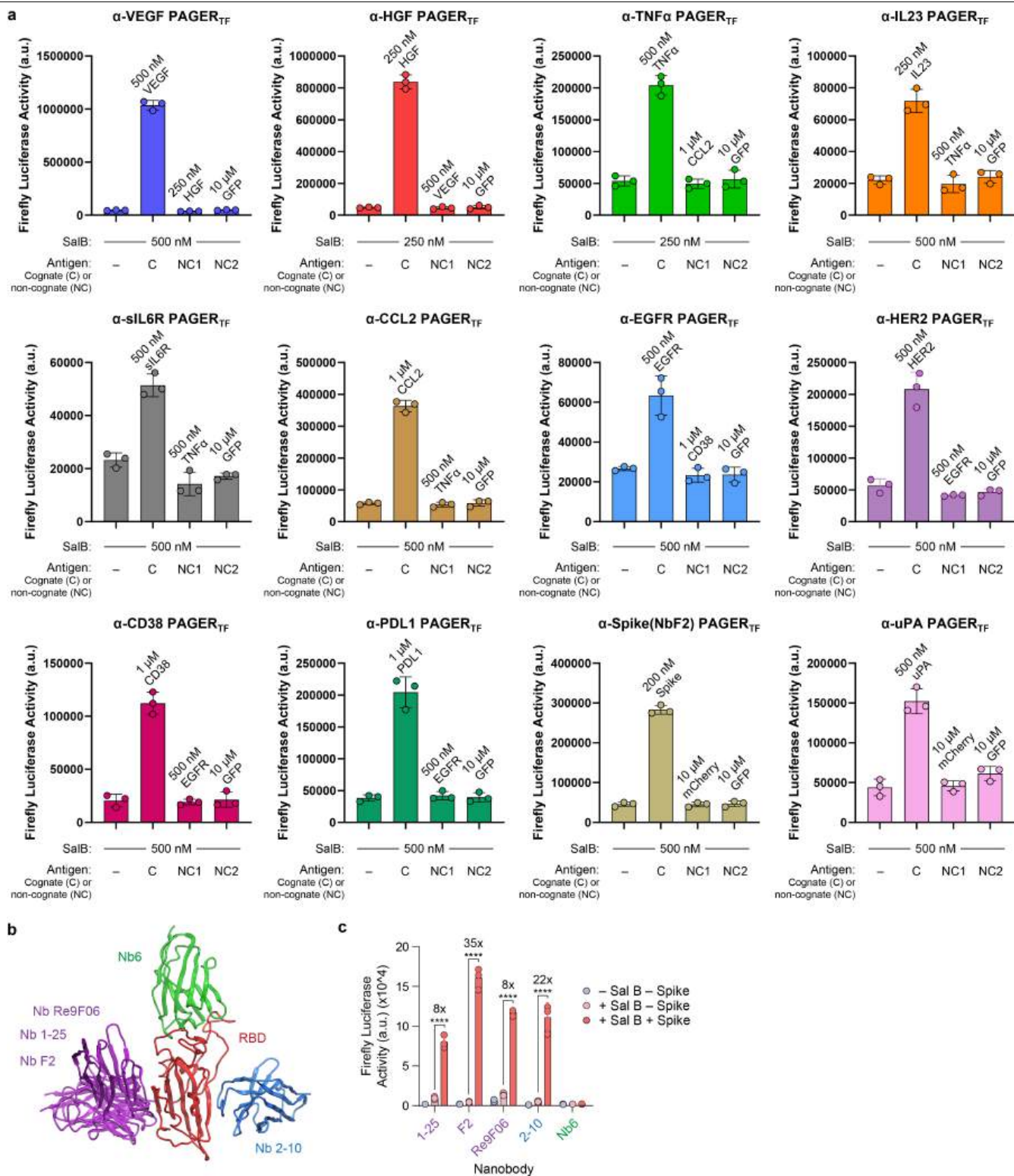
Extended Data Fig. 5 | PAGER TF detects a wide range of antigens (Related to Fig. 2a). a , PAGER TF antigen response assay. Same as Fig. 2a, but including comparisons of cognate antigen to two non-cognate antigens for each PAGER TF . The antigens used and their concentrations are labeled above each bar. Plots are mean \pm s.d. for 3 technical replicates per condition, n = 1 independent experiment. b , Five nanobodies that bind to the receptor binding domain (RBD) of SARS-CoV2 spike protein as shown (sequences in Supplementary Information)
