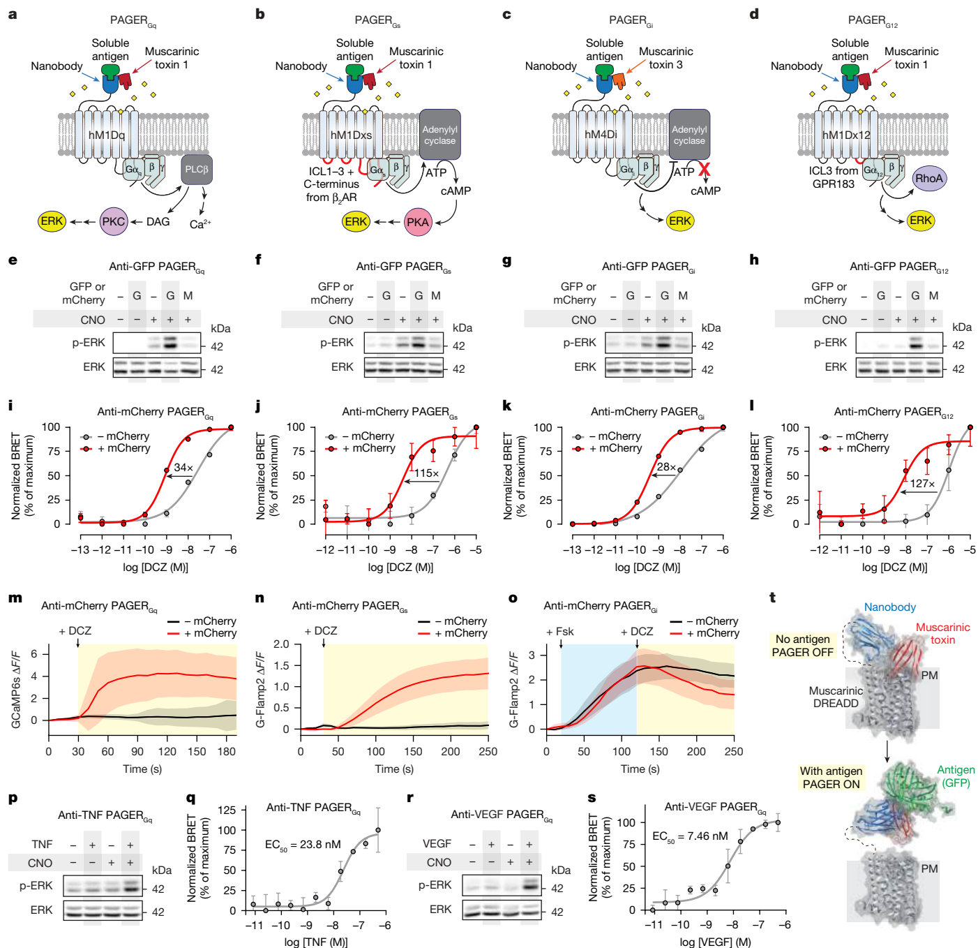
Fig. 3 | PAGER G couples antigen recognition to activation of endogenous G-protein signalling. a–d , Schematics for PAGER Gq ( a ), PAGER Gs ( b ), PAGER Gi ( c ) and PAGER G12 ( d ), showing designs and downstream signalling induced by their activation. β 2 AR, β 2 -adrenergic receptor. e–h , Western blots showing phosphorylation of ERK (p-ERK) in response to activation of PAGER Gq ( e ), PAGER Gs ( f ), PAGER Gi ( g ) and PAGER G12 ( h ). G and M indicate GFP and mCherry, respectively. HEK cells were stimulated with 100 nM CNO and 1 μM GFP for 5 min before analysis. n = 3 independent experiments. i–l , DCZ dose–response curves for PAGER Gq -mediated ( i ), PAGER Gs -mediated ( j ), PAGER Gi -mediated ( k ) and PAGER G12 -mediated ( l ) G-protein activation using TRUPATH BRET assay. HEK cells were stimulated with 1 μM mCherry. n = 4 independent experiments, 3 replicates per condition. Data are mean ± s.d. m–o , Representative kinetic measurements of second messenger levels in HEK cells expressing anti-mCherry PAGER Gq ( m ), PAGER Gs ( n ) or PAGER Gi ( o ). The calcium indicator GCaMP6s (for PAGER Gq ) or the cAMP indicator G-Flamp2 (for PAGER Gs and PAGER Gi ) were
