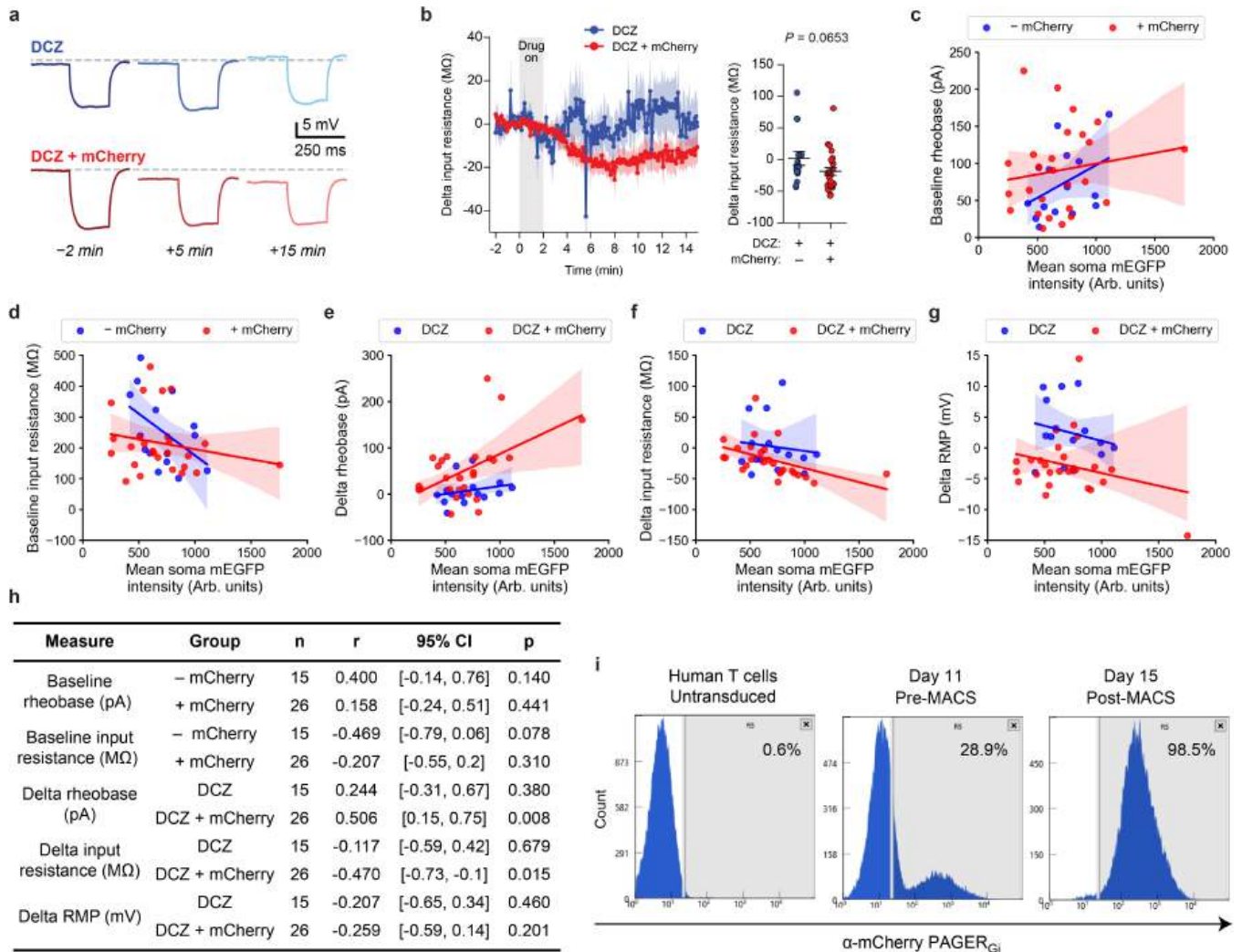
Extended Data Fig. 12 | PAGERG 1 expression in acute brain slices and primary T cells. a , Representative traces of voltage responses to -100 pA stepwise current injections relative to onset of 2 min bath application of DCZ (100 nM) \pm soluble mCherry (1 \mu M). Dashed line at -65 mV. b , Changes in input resistance upon 2-minute DCZ addition. n = 15 cells/7 animals DCZ, n = 26 cell/6 animals DCZ+mCherry. Plots show mean \pm S.E.M. (Mixed linear model regression analysis; Z = 1.84 , P = 0.0653 ). c-h , Correlation between PAGERG 1 -associated mEGFP expression and neuronal intrinsic properties. The degree of mEGFP expression, as an indicator of PAGERG 1 expression levels in neurons, supports PAGERG 1 alone having no impact on baseline rheobase (c) or input resistance (d) properties, including in the presence of soluble mCherry. Construct expression
